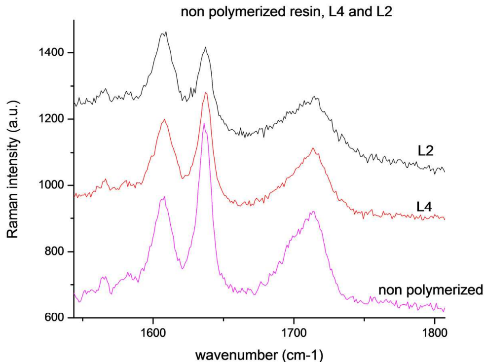
Fig. 5. Raman test results for Elipar polymerization device and thicknesses of 2 mm (L2-G2) and 4mm (L4-G4)
