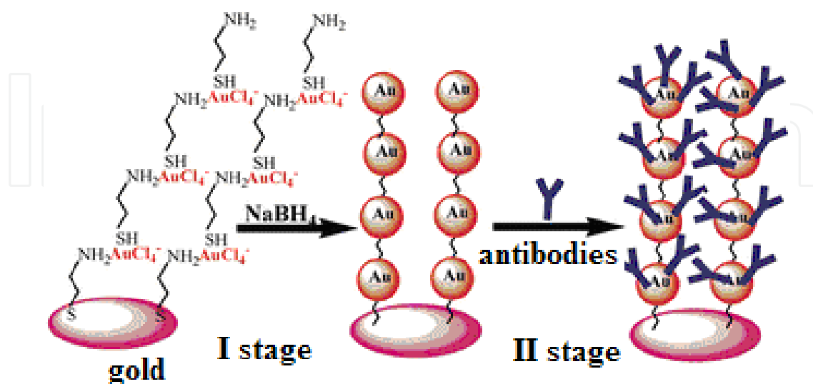
Fig. 7. The formation of the receptor layer on the surface of the gold electrode: Stage I - nano-chains generation of molecules HAuCl 4 and AET; Stage II - immobilization of antibodies (Tang et al. 2008).
