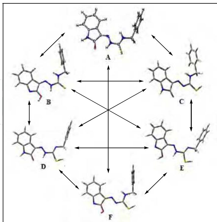
Fig. 2. Possible tautomeric forms for compound 18
