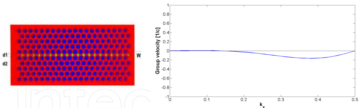
Fig. 12. Optimized photonic crystal waveguide on a triangular lattice of air holes on silicon with d_1=0.51 \cdot a , d_2=0.76 \cdot a , W=0.64 \cdot W (left) and group velocity of the defect mode (right)
