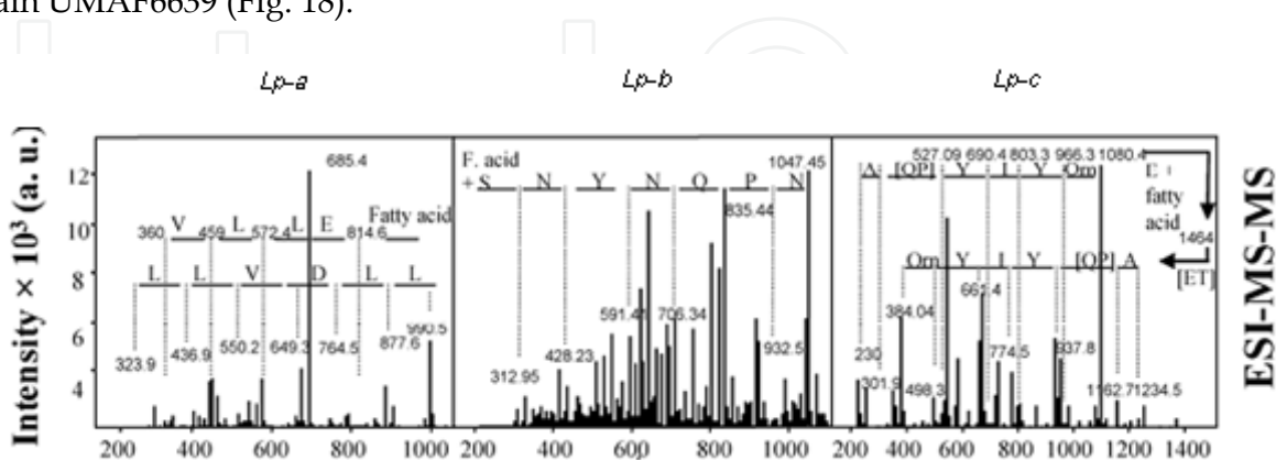
Fig. 18. Mass spectra scored for the purified fractions LP-a, LP-b, and LP-c.
