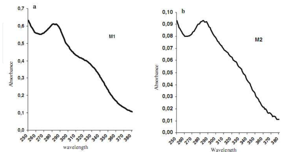
Fig. 8. UV absorption spectra between 250 and 280 nm wavelengths a: peak one, b: peak two.
