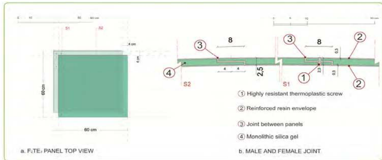
Fig. 11. F 2 TE 3 Envelope Profile Design
