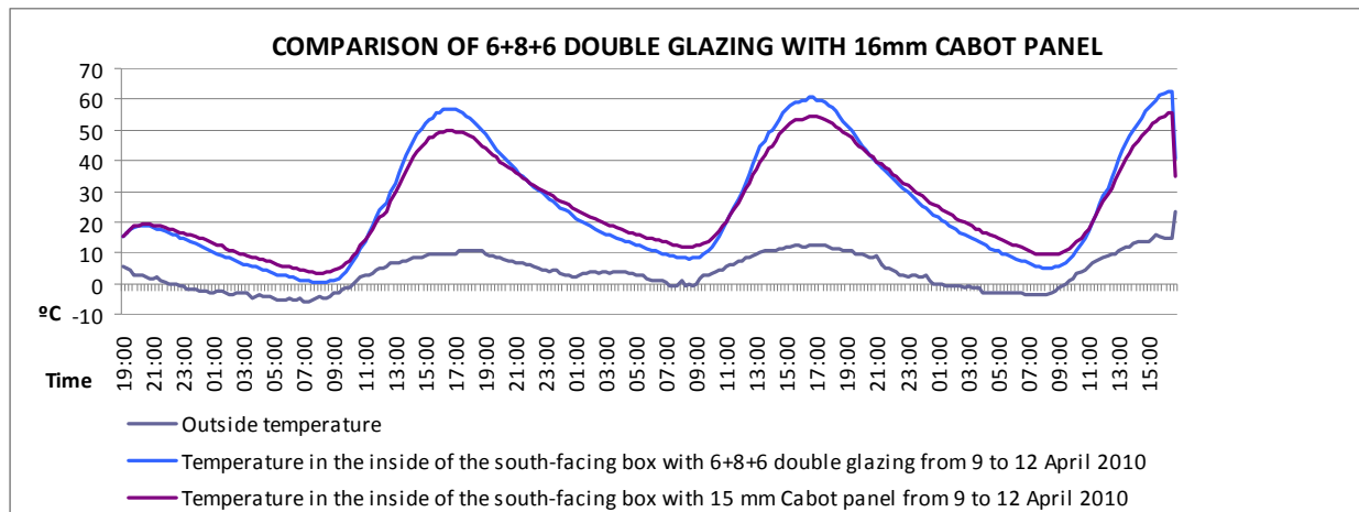
Fig. 6. Trial 1. Sample tested: (600x600mm of side) Polycarbonate Panel of 16mm thick filled with nanogel. The test was made from the 9th (19:00 h) to 12 (15:00 h) in April 2010. At the E.T.S.A.M. School of Architecture & School of Computing (UPM) Spain
