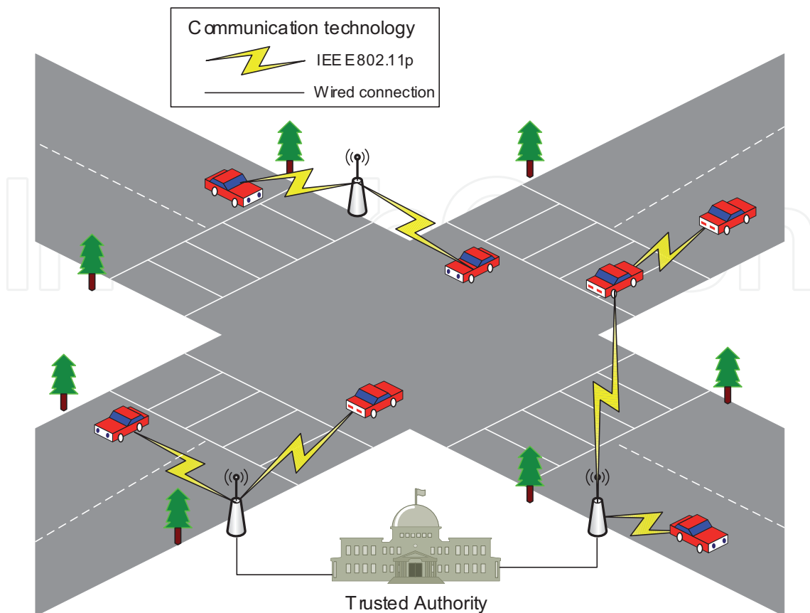
Fig. 2. VANETs Architecture
