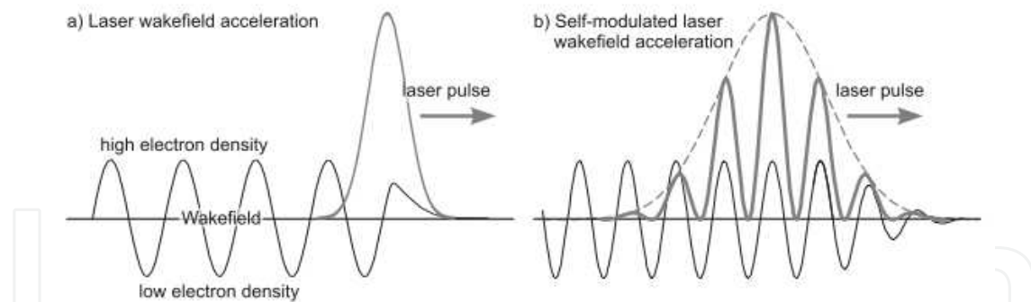
Fig. 2. Laser envelope and electron density schematic in the laser wakefield regime (a) and in the self-modulated wakefield regime.
