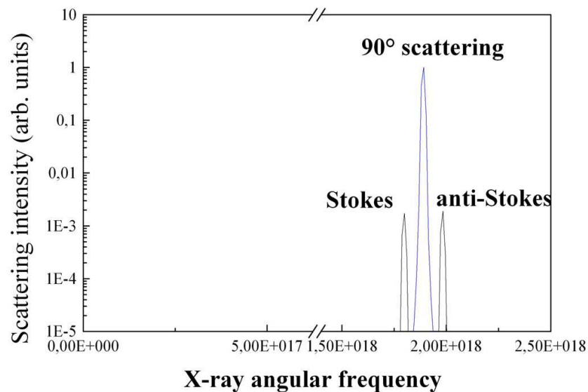
Fig. 10. Result of an exact numerical calculation of the scattering spectrum of a 10 MeV electron, chosen at random in a 1 \mu\text{m} normalized emittance bunch focused over 30 \mu\text{m} rms, and injected into the transverse light lattice.
