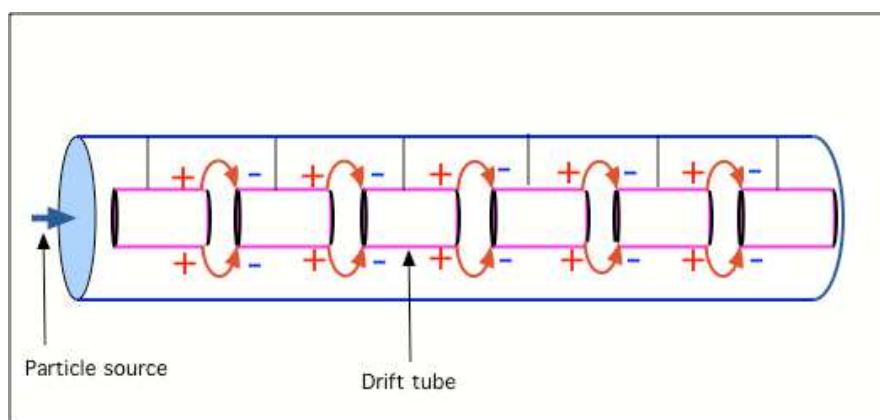
Fig. 1. Linear Particle Accelerator schematic.
