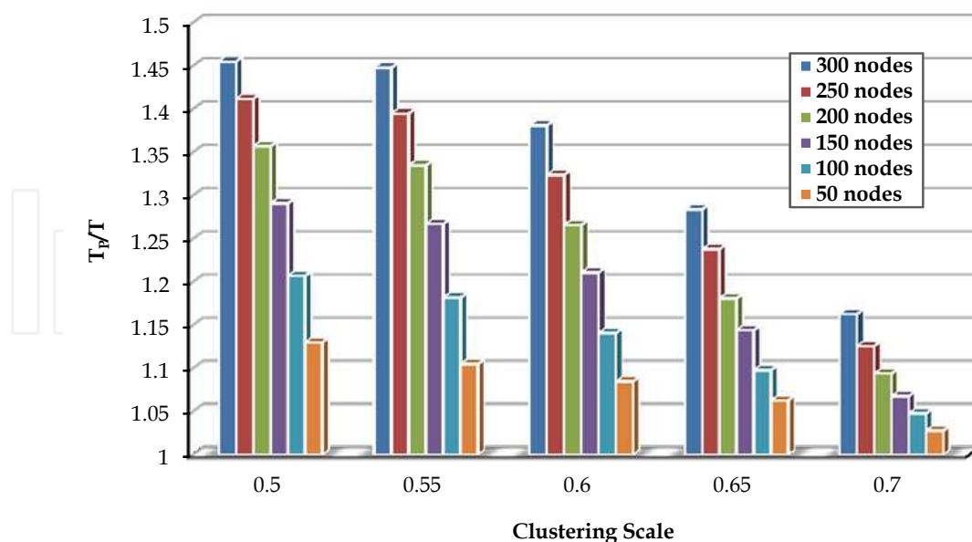
Fig. 8. T_P/T for several node densities and clustering scales.
