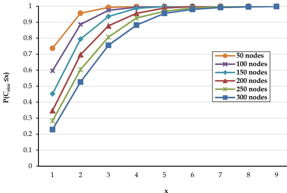
Fig. 5. The cluster size cumulative distribution function ( \gamma = 0.5 ).
