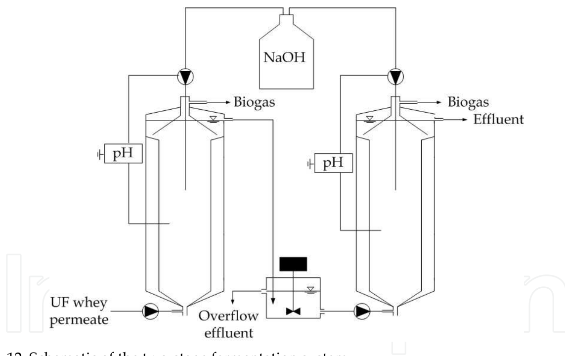
Fig. 12. Schematic of the two-stage fermentation system
