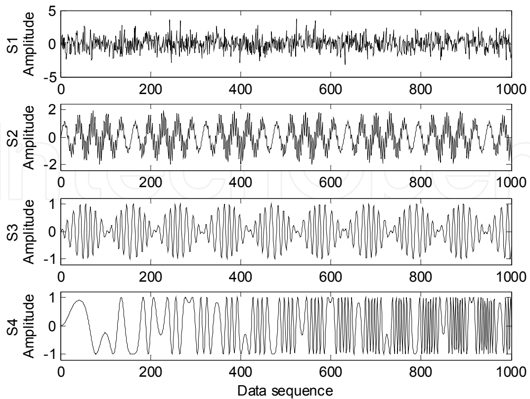
Fig. 2. Waveforms of the source signals
