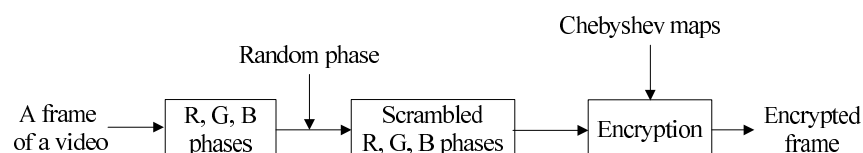
Fig. 9. The video encryption scheme in(Ganesan et al., 2008)
