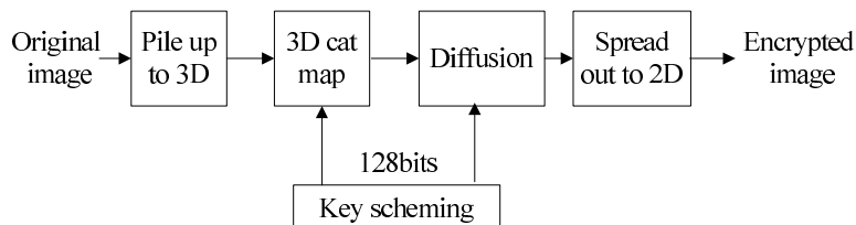
Fig. 5. The image encryption scheme in (Chen et al., 2004)
