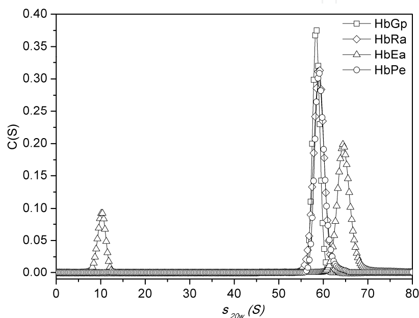
Fig. 4. Continuous sedimentation coefficient distribution of extracellular hemoglobins. The c(S) fittings for hemoglobins, at a concentration of 200 \mu\text{g/mL} , in 100 mmol/L Tris-HCl containing 50 mmol/L NaCl, are shown. The s_{20,w} for each fitted curve was determined as the maximum of the peaks of c(S) curves. Absorbance was monitored at 415 nm.
