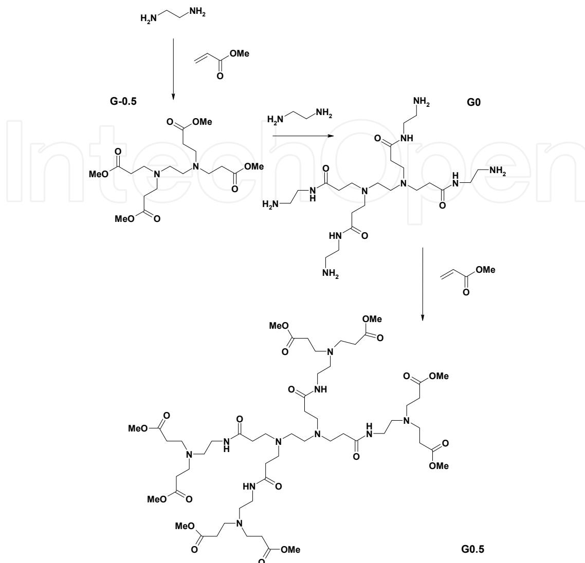
Scheme 1. The scheme of synthesis of PAMAM dendrimers on ethylenediamine (en) core. Addition of methyl acrylate to en results in formation of -0.5 half-generation PAMAM dendrimer (G-0.5) with four methyl ester groups on surface. The condensation of G-0.5 with four en equivalents leads to full-generation PAMAM dendrimer (G0). Further addition of methyl acrylate gives G0.5 PAMAM dendrimer, which upon next condensation with eight en equivalents results in obtaining full generation PAMAM dendrimer G1 (not shown). Repeated sequence of addition/condensation protocol leads to G1.5, G2, G2.5, G3 and so on.
