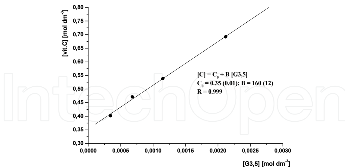
Fig. 2. The dependence of solubility of 1 in methanol containing variable concentration of G3.5.
