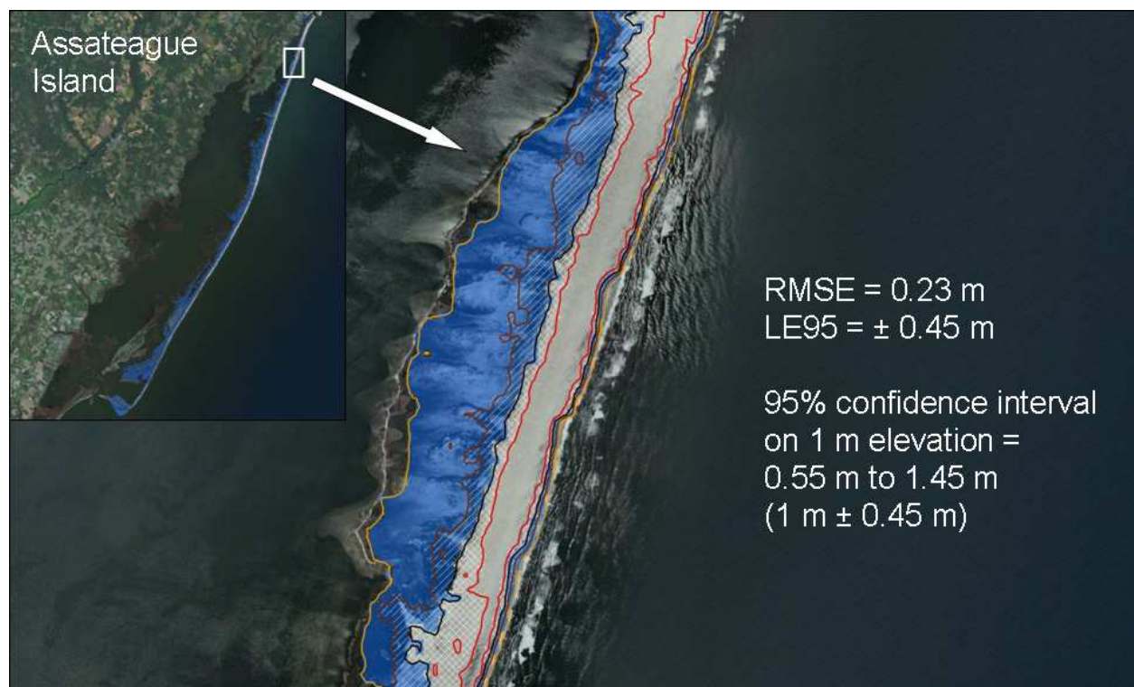
Fig. 2. Results of an accuracy assessment of lidar elevation data over a portion of Assateague Island. The orange line is the mean high water (MHW) shoreline. The black line is the 1-meter contour (above MHW), and the brown lines and cross-hatch patterns delineate a buffer around the 1-meter elevation. This buffer represents a spatial projection of the area of uncertainty associated with the 1-meter elevation (the 95% confidence interval, or 1 \text{ m} \pm 0.45 \text{ m} ). The blue tint covers the area between the MHW shoreline and the 1-meter elevation. The background is an orthoimage.
