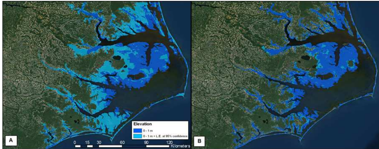
Fig. 1. Lands vulnerable to a 1-meter sea-level rise, developed from topographic map-derived DEMs (A) and lidar elevation data (B). The darker blue tint represents the area at or below 1 meter in elevation, and the lighter blue tint represents the additional area in the vulnerable zone given the vertical uncertainty of the input elevation datasets. The background is a true color orthoimage.
