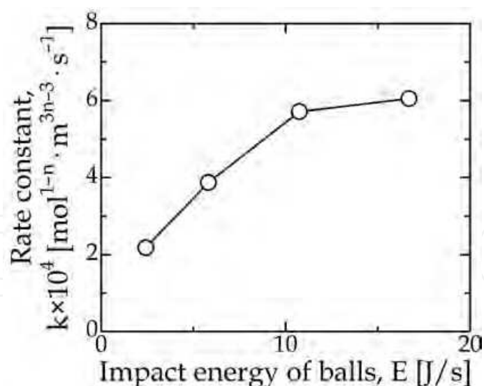
Fig. 14. Relationship between rate constant k and impact energy E of balls per unit time.
