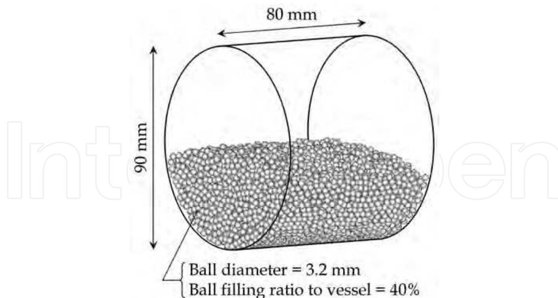
Fig. 1. Schematic illustration of tumbling ball mill used in this work.
