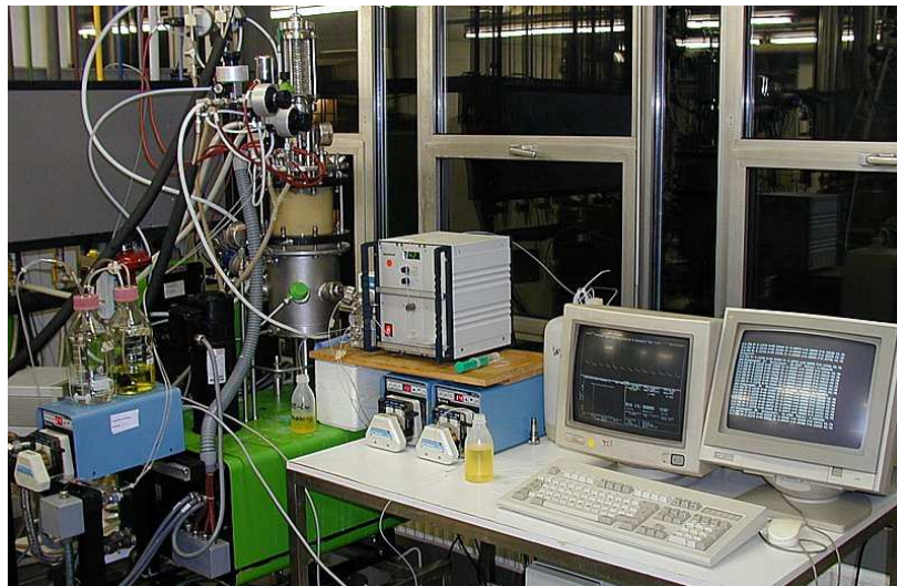
Fig. 1. Experimental equipment
