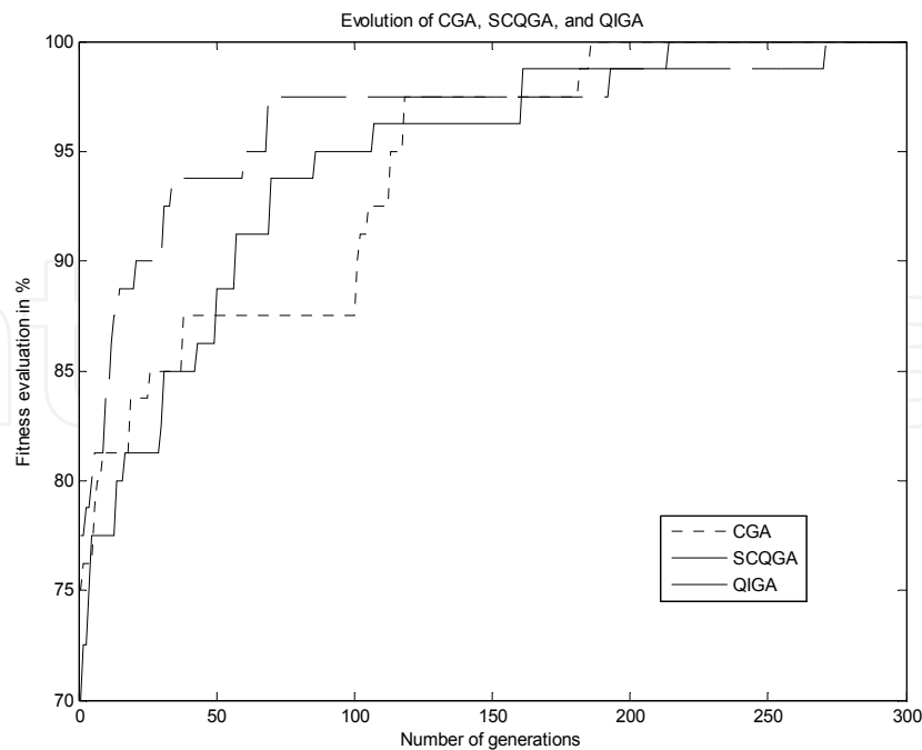
Fig. 10. The evolutions of CGA, SCQGA and QIGA
