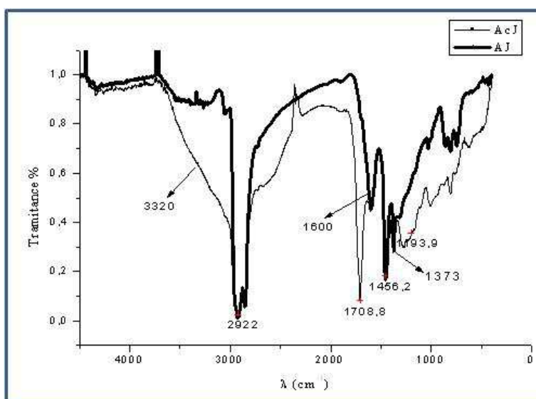
Fig. 1. Comparison of AcJ and AJ FTIR spectra.
