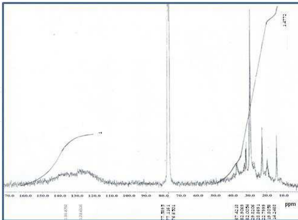
Fig. 4. ^{13}\text{C} NMR spectrum for AJ.
