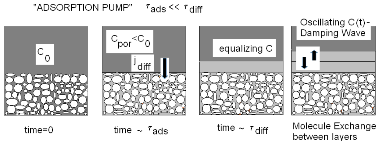
Fig. 7. "Adsorption Pump". Comments are in the text.
