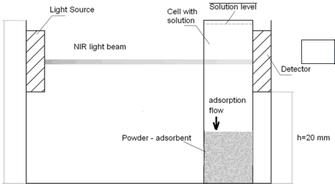
Fig. 1. Experimental setup for measuring adsorption on powders.
