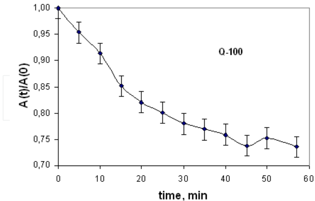
Fig. 3. Time change of integral transmittance of asphaltene solution (normalized to a value in initial time point). Sample Q-100.
