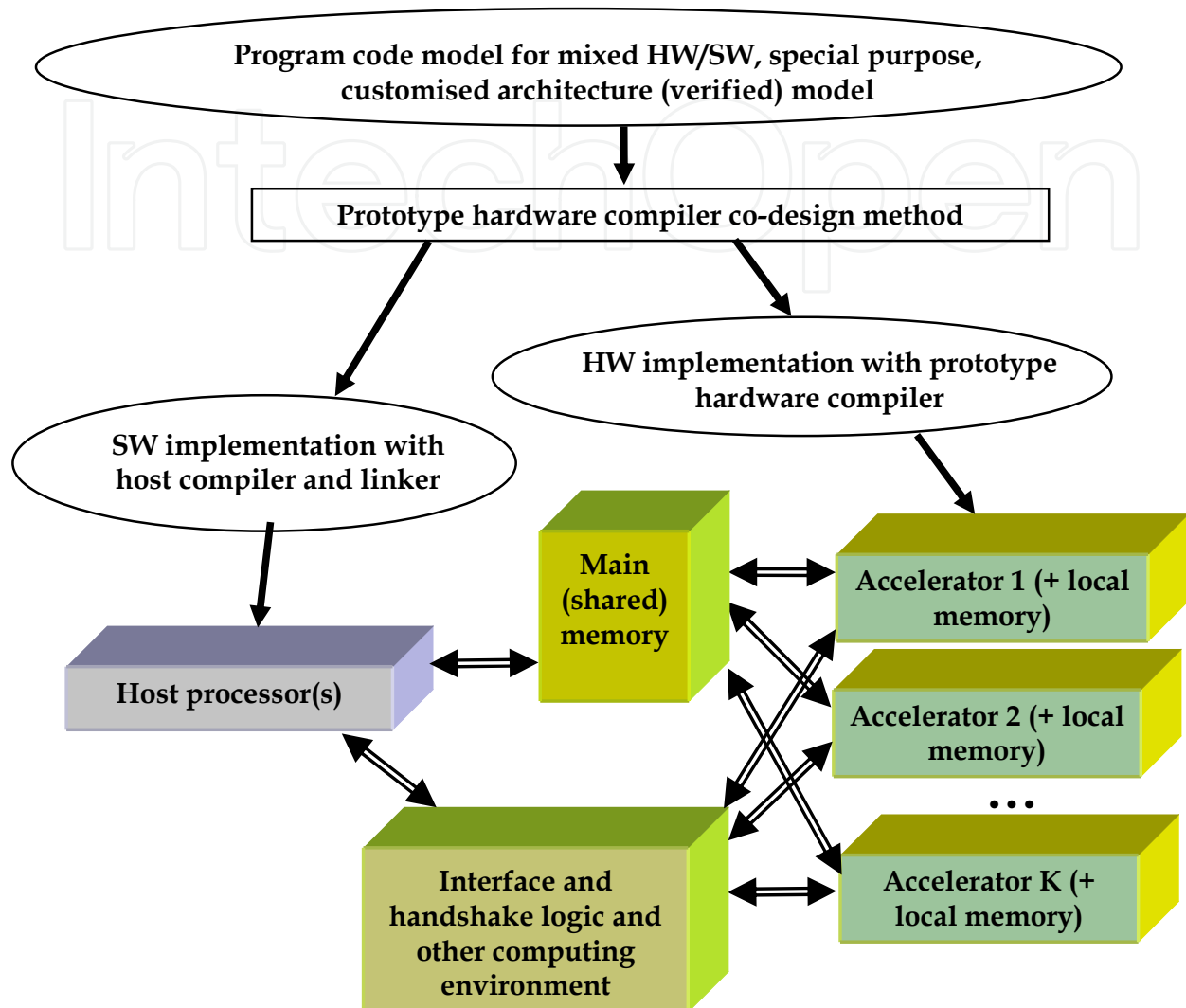
Fig. 7. Host computing environment and accelerators execution configuration.
