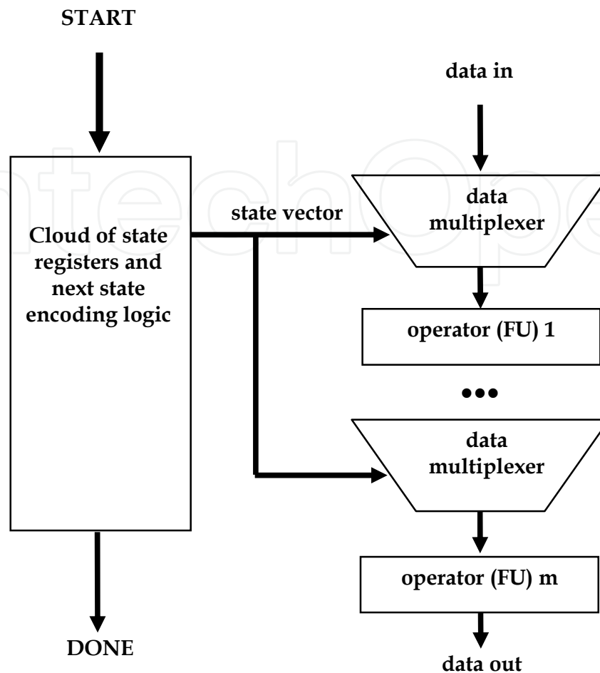
Fig. 6. The traditional FSM + datapath generated micro-architecture option.
