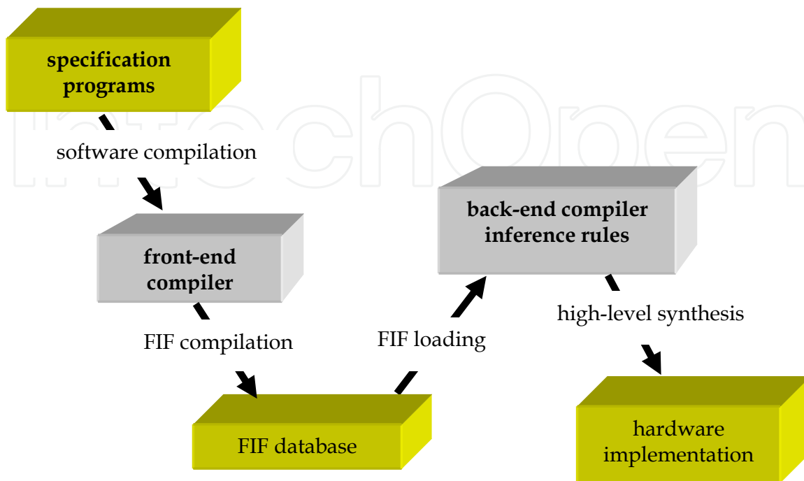
Fig. 1. Hardware synthesis flow and tools.
