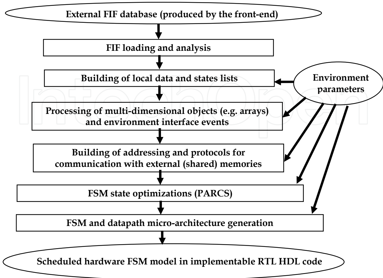
Fig. 3. The processing stages of the back-end compiler.
