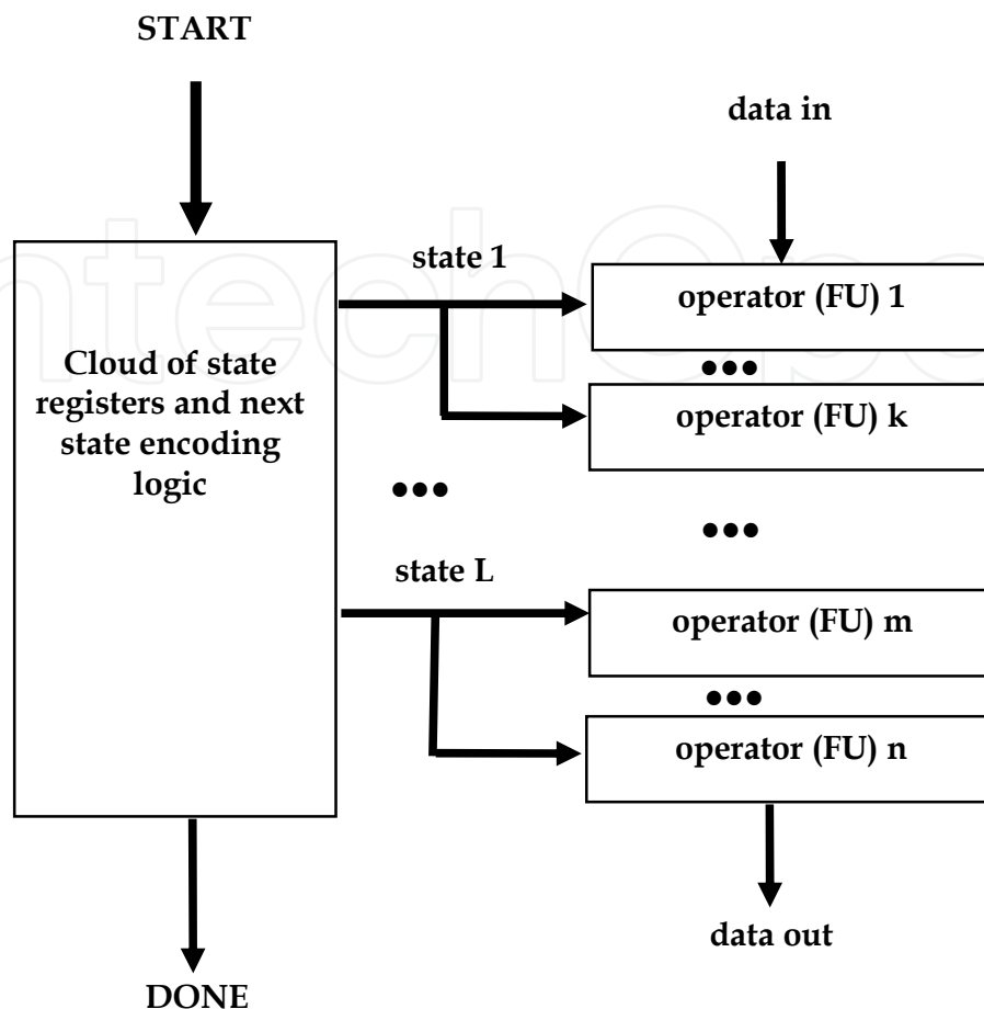
Fig. 5. Massively-parallel microarchitecture generation option.
