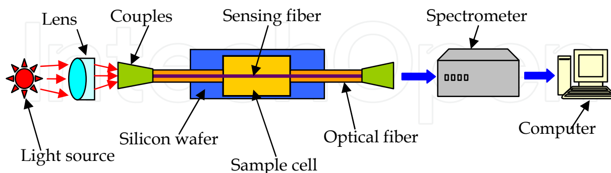
Fig. 14. The experimental set-up
