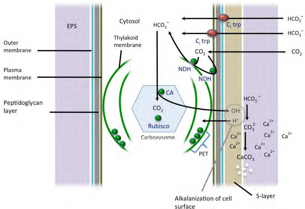
Fig. 6. Model of the carbon concentrating mechanism (CCM) and calcification in a cyanobacterial cell. \text{CO}_2 enters the cells mainly via active transport of \text{HCO}_3^- but also through diffusion of \text{CO}_2 , which is converted to \text{HCO}_3^- during the uptake. Cytosolic \text{HCO}_3^- is subsequently imported to the carboxysome. CA, carbonic anhydrase; \text{C}_i , inorganic carbon; EPS, exopolysaccharide substances; NDH, NADPH dehydrogenase; PET photosynthetic electron transport. Modified from Jansson and Northen.
