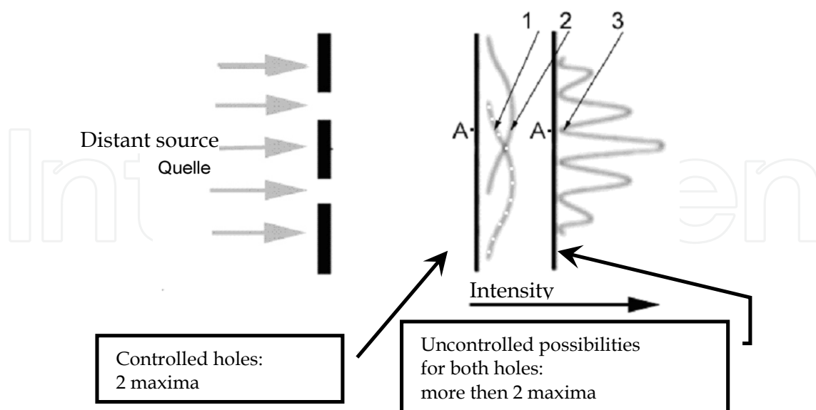
Fig. 3. When quantum particles have the possibility to go through both slits without controlling their passage, then one will find more than two maxima on a screen behind the slits. Position “A” can be reached if one of the holes is open, but no longer if both are open and not controlled.
