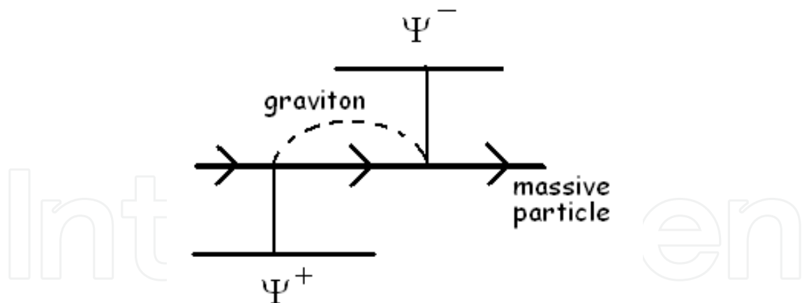
Fig. 7. Zero-mode excitation by double interaction with incoherent matter. A single massive particle can cause such an excitation by emitting and re-absorbing a virtual graviton, but the probability of this process is very small.
