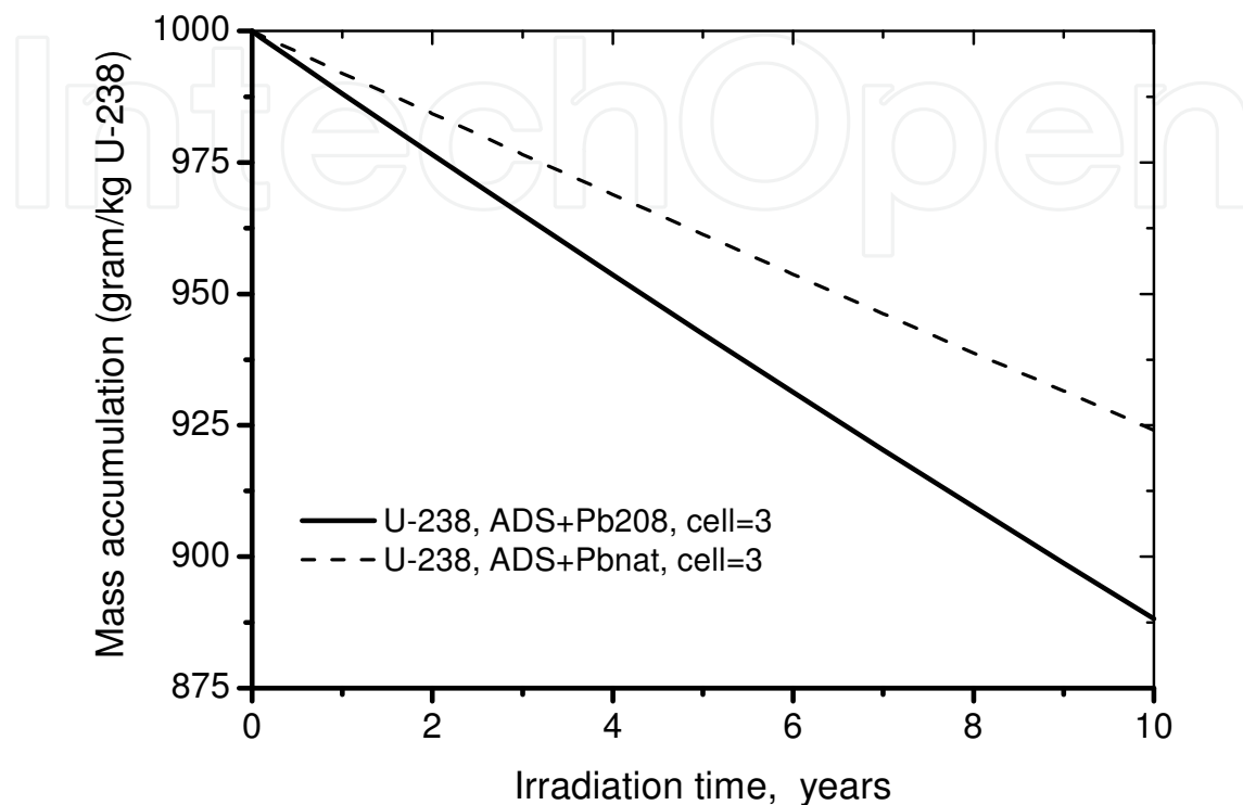
Fig. 7. Mass burning of 1 kg of U-238 in the neutron spectra of 80 MW ADS blanket, in the cell 3 which is near far blanket's margin. The solid curve corresponds to the case, when the blanket is cooled with lead-208, the dash curve - to the case, when the blanket is cooled with lead natural.
