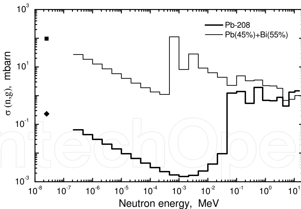
Fig. 2. Microscopic cross sections of radiation neutron capture s(n,g) by stable lead-208 isotope and by the eutectic Pb-nat(45%) - Bi (55%) taken from the ENDF/B-VII.0 library. Cross sections are represented in the ABBN-93 system of 28 neutron energy groups.
