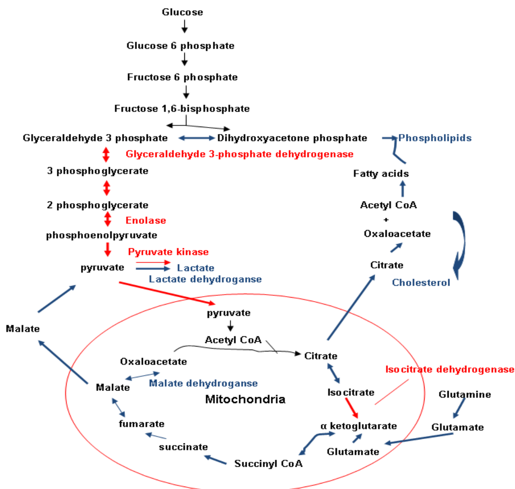
Fig. 3. Metabolic model of the adaptation of NS0 cell line to protein free-medium obtained from proteomic and metabolites analysis. Red: sub-expressed pathways. Blue: over-expressed pathways.
