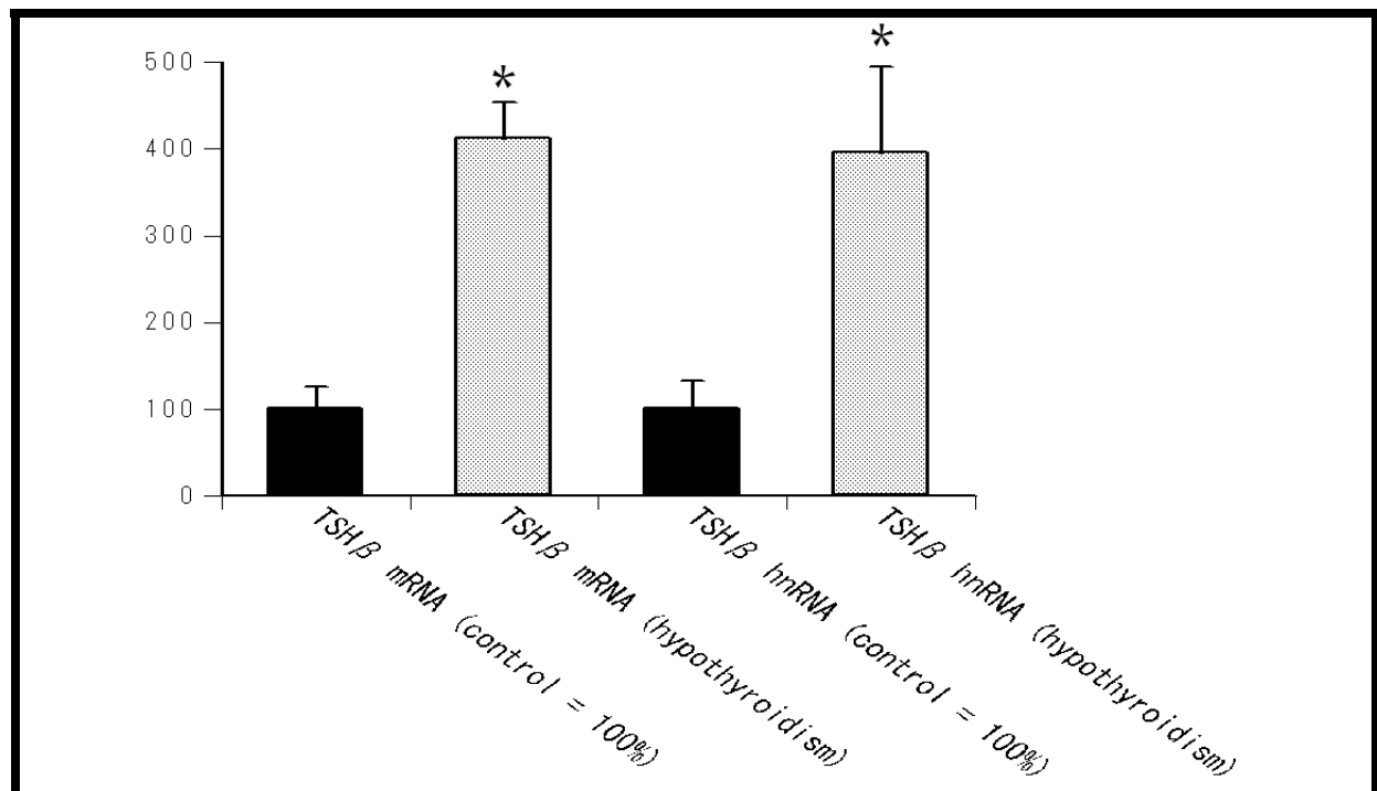
Fig. 4. Detection of the RT-PCR amplicons for TSH \beta mRNA and hnRNA by thermal cyclor
