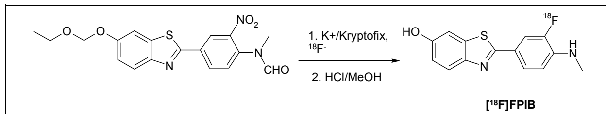
Scheme 3. Synthesis of [ 18 F]flutemetamol ([ 18 F]FPIB)
