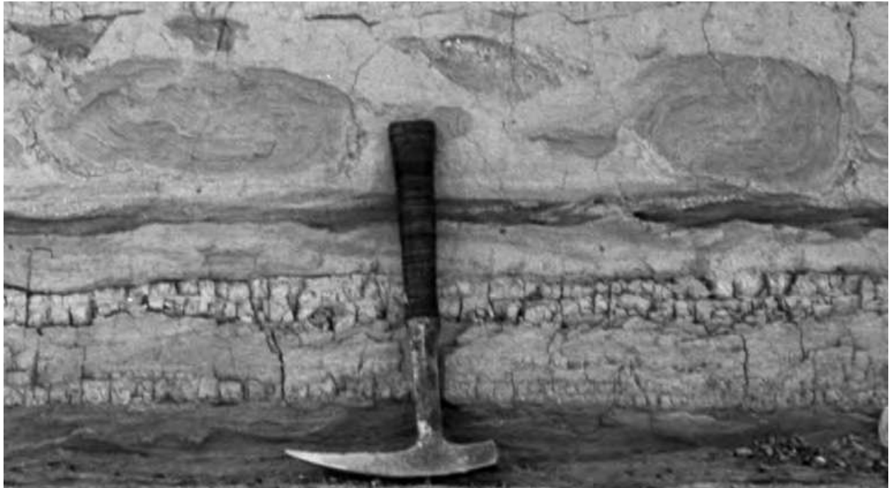
Fig. 4. Ball and pillow structures observed in silty and sandy lacustrine deposits of Lake Van.
