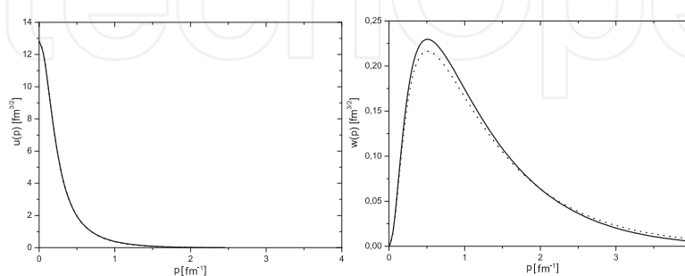
Fig. 3. Deuteron wave functions \psi_0^d(p) = u(p) and \psi_2^d(p) = w(p) . Solid(dotted) curves for Bonn Potential B (UCT) potential.
