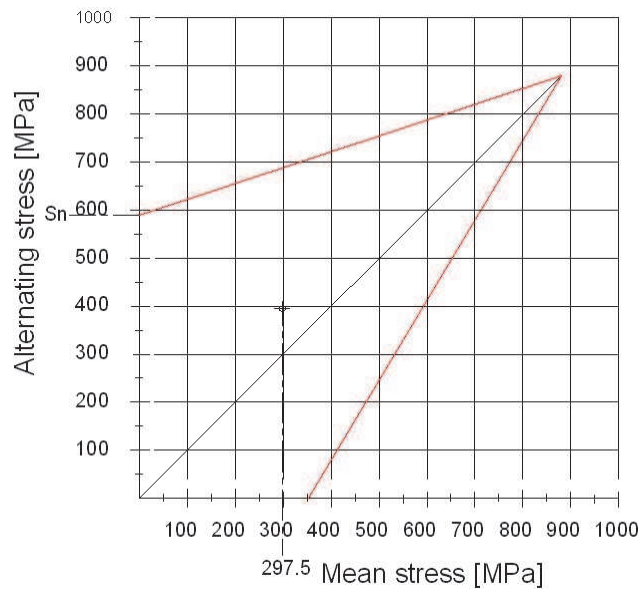
Fig. 4. Goodman's diagram. Ti6Al4V
