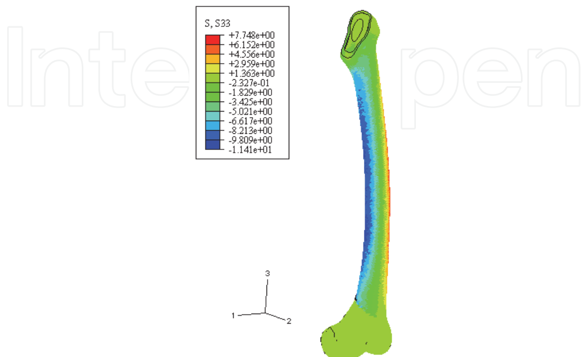
Fig. 6. S33 Stress in the bone, stemmed Ti35Nb7Zr5Ta implant model
