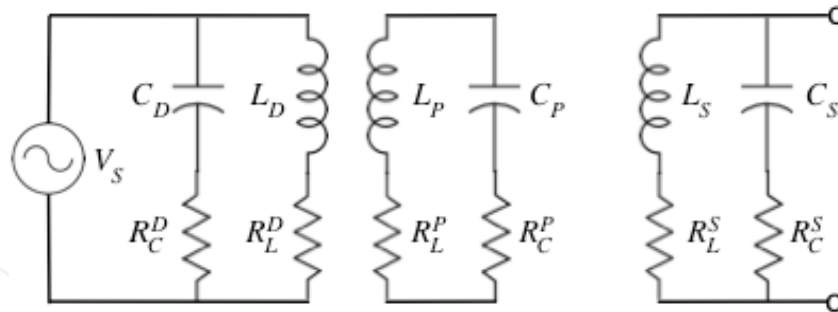
Fig. 3. Electrical model of drive, primary and secondary coils.
