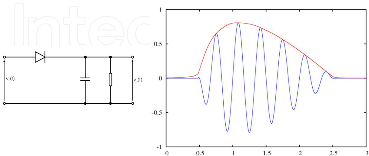
Fig. 6. Envelope detector circuit (left) and the resulting ideal envelope (right).
