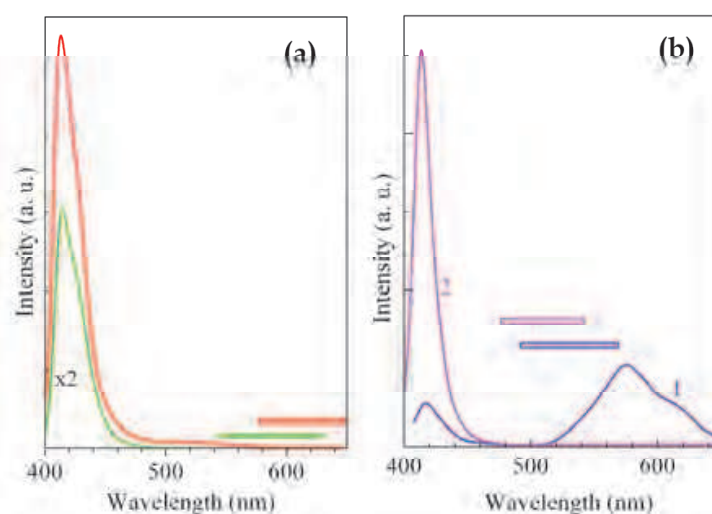
Fig. 11. Emission spectra of two different initial opals after thermal annealing at 800 °C (a). Emission spectra of opal conserved for a long time in the air at 70 % moisture (b) before (1) and just after (2) annealing at 700 °C. The rectangles point to the stop-band positions.
