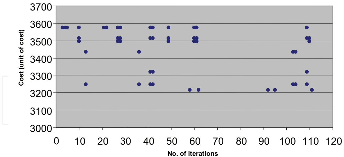
Fig. 5. Bids received at each TS move ( \alpha = 30\% ).
