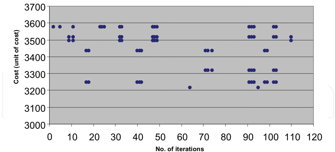
Fig. 3. Bids received at each TS move ( \alpha = 15\% ).
