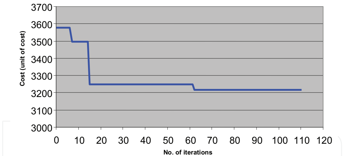
Fig. 4. Optimum bid recorded at each TS move ( \alpha = 15\% ).
