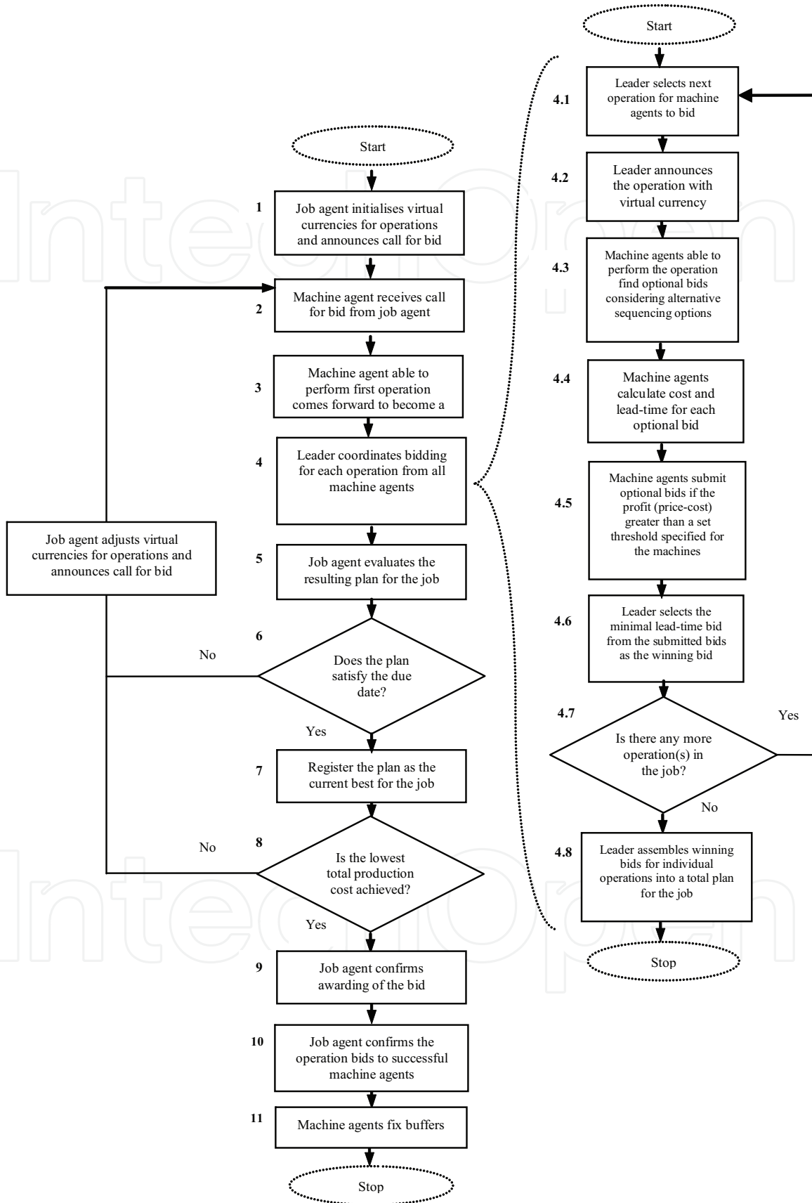
Fig. 1. Iterative agent bidding mechanism
