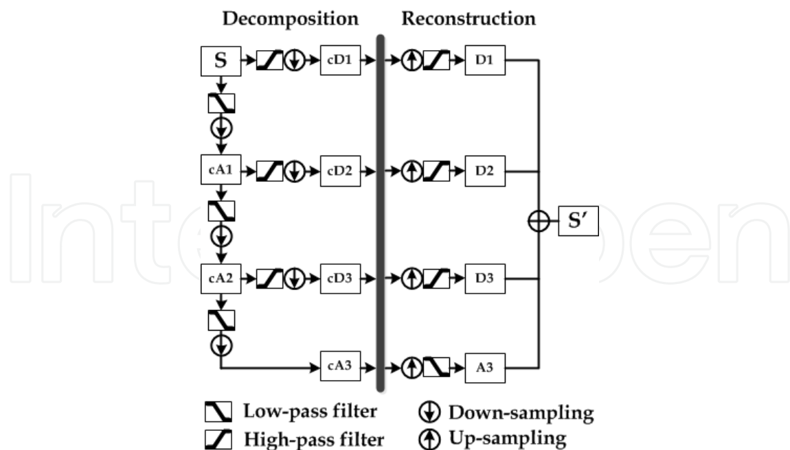
Fig. 1. Wavelet decomposition and reconstruction process.
