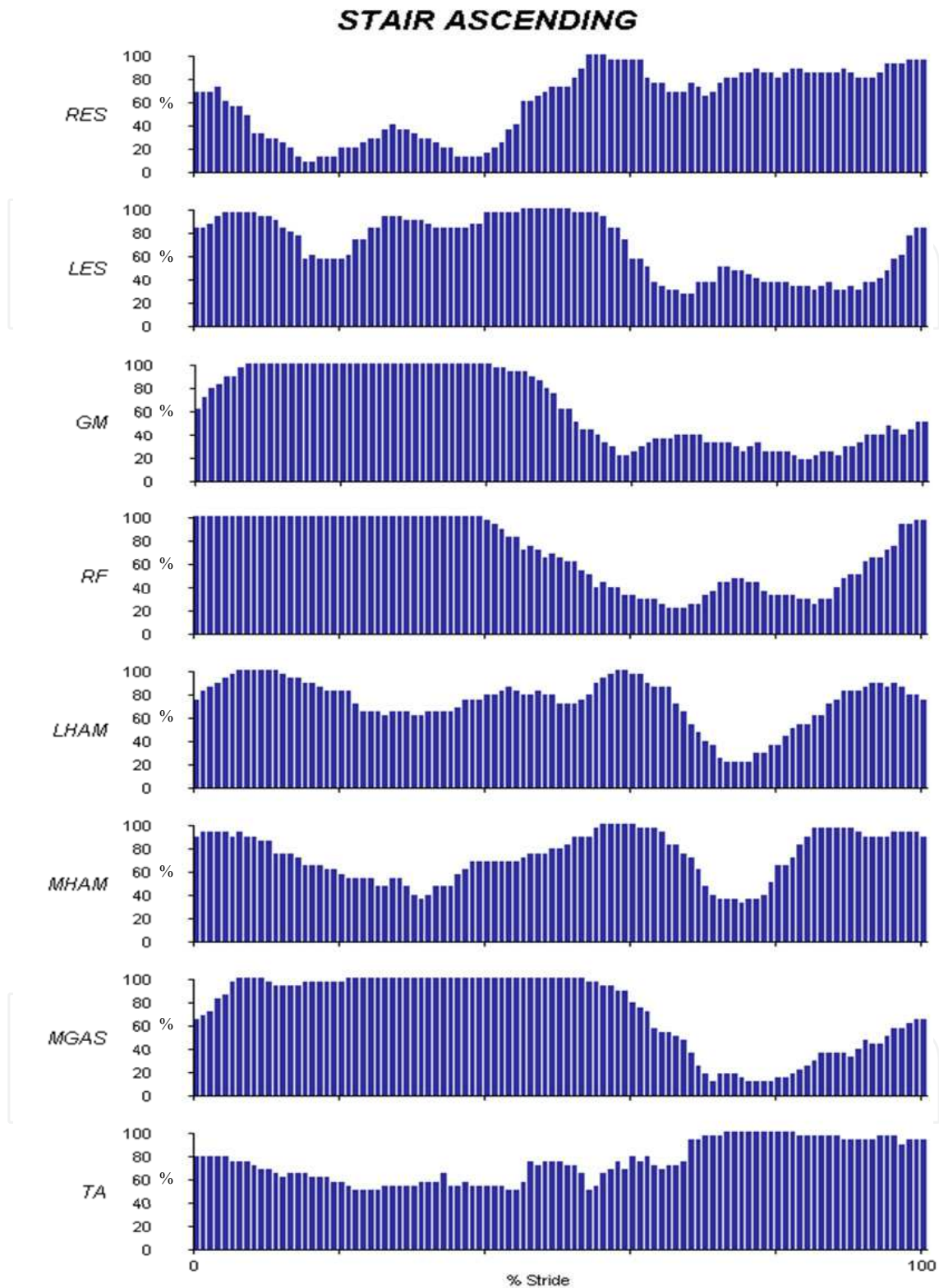
Fig. 3. On-off muscle timing during stair ascending, as a function of the percentage of the gait cycle. For each muscle, the muscular activity is presented as percentage of subjects whose muscle is active at the specific percent of the stride considered. RES: right erector spinae, LES: left erector spinae, GM: gluteus medius, RF: rectus femoris, MHAM: medial hamstrings, LHAM: lateral hamstrings, MGAS: medial gastrocnemius, TA: tibialis anterior.
