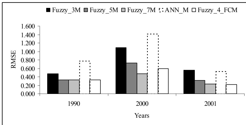
Fig. 2. Performance comparison of models.
