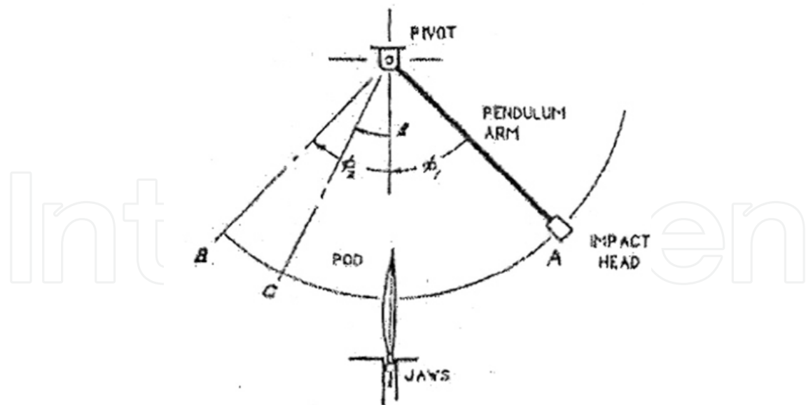
Fig. 3. Arrangement and analysis of pendulum (from Liu et al. , 1994).
