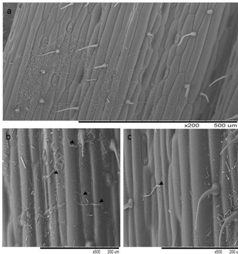
Fig. 5. Electron microscopic exposures of Dinosor leaves sampled at 15 dpi by a 10 \mu l-drop of M. graminicola conidiospores 10^5 \cdot \text{ml}^{-1} : (a) nontreated control, where almost all spores germinated and stomata near from the point of inoculation were penetrated; and (b and c) wheat leaf treated with prothioconazole one day before inoculation (d-1), where spores failed to germinate and almost all spores degraded.
