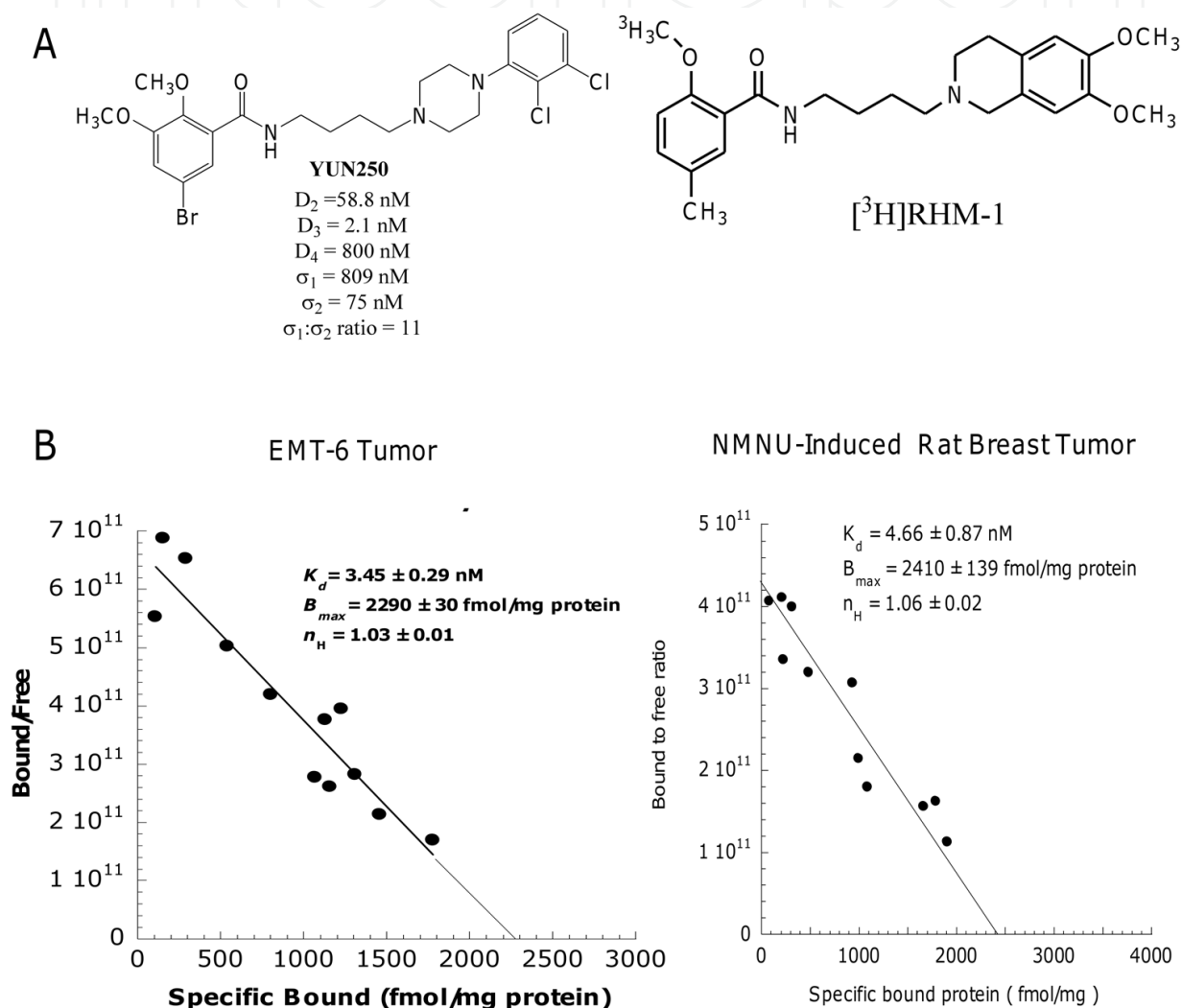
Fig. 3. The conformationally-flexible benzamide-based \sigma_2 receptor ligands for in vitro studies of the \sigma_2 receptor. A: YUN250 was a lead for generating the conformationally-flexible benzamide analogues which are selective for \sigma_2 receptors. The tritium labeled ligand, [ 3 H] RHM-1 , has been used to conduct the receptor binding assay. B: Scatchard studies of \sigma_2 receptors in EMT-6 mouse breast tumors and NMNU-induced rat breast tumors with [ 3 H] RHM-1 . This probe has high affinity to the \sigma_2 receptors in the rodent breast tumors and is useful for in vitro binding studies.
