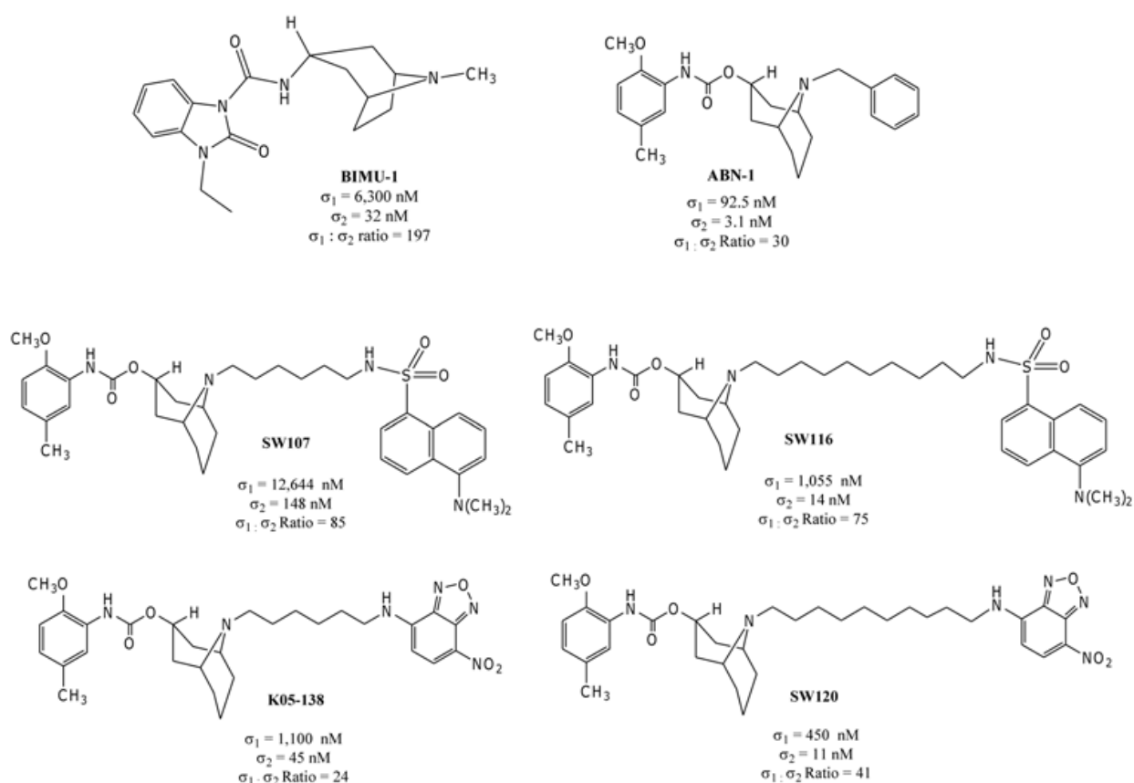
Fig. 2. Structures of BIMU-1 and the granatane analogs. ABN-1 was used as a lead for producing second-generation granatane-based \sigma_2 receptor ligands, which led to the development of a number of fluorescent probes, K05-138 , SW120 , SW107 and SW116 , for two photon and confocal microscopy studies of \sigma_2 receptors in tumor cells.
