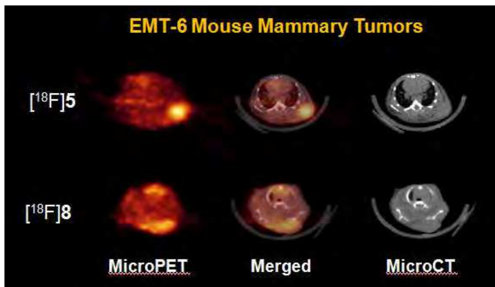
Fig. 4. The synthetic schemes for generating conformationally-flexible benzamide-based PET radiotracers. A: A number of ^{11}\text{C} -labeled radiotracers, [ ^{11}\text{C} ] 1-4 , are prepared by labeling the corresponding ortho-hydroxy group with [ ^{11}\text{C} ]methyl iodide. B: A number of ^{18}\text{F} -labeled radiotracers, [ ^{18}\text{F} ] 5-8 , are generated by replacing of the 2-methoxy group in the benzamide ring with a 2-fluoroethoxy group. C: Biodistribution studies in female Balb/c mice bearing EMT-6 tumor allografts demonstrating that all four ^{18}\text{F} -labeled compounds had a high tumor uptake (2.5-3.7% ID/g) and acceptable tumor/normal tissue ratios at 2 h post-i.v. injection. D: MicroPET imaging studies indicate that [ ^{18}\text{F} ] 5 and [ ^{18}\text{F} ] 8 are suitable probes for imaging the \sigma_2 receptor status of solid tumors with PET.
