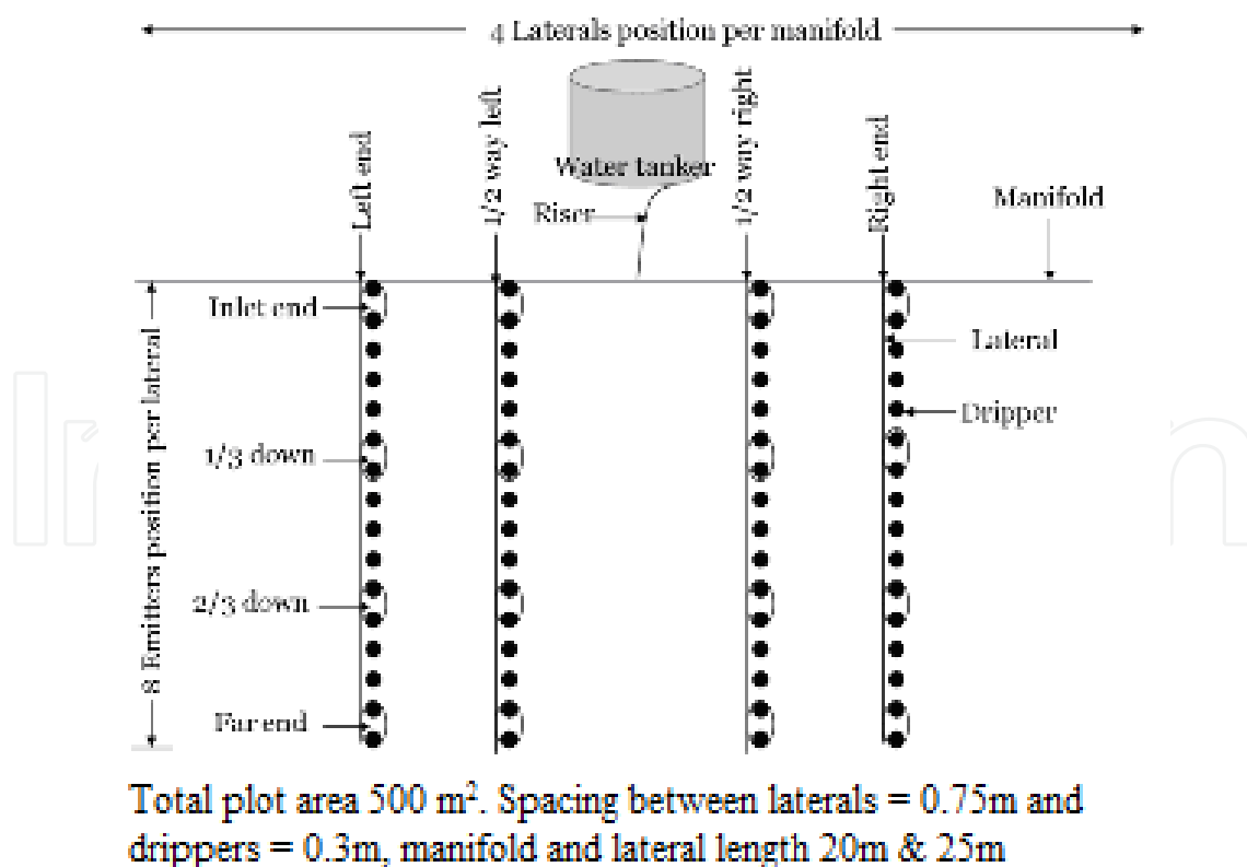
Fig. 3. Layout of control points and discharge measurement for family drip irrigation system of this study
