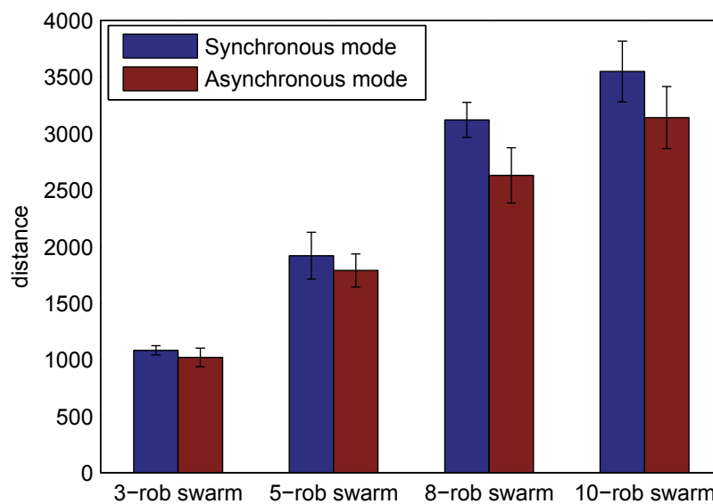
Fig. 9. Average total distance passed by all robots for 10 runs search success under conditions of R_{detec} = 125, R_{comm} = 250 .
