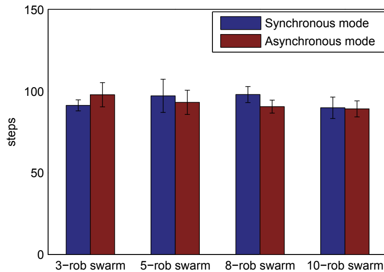
Fig. 8. Average time steps required to complete target search for 10 runs under conditions of R_{detec} = 125, R_{comm} = 250 .
