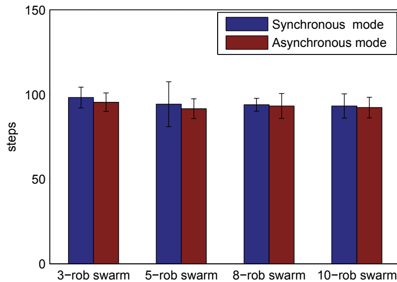
Fig. 6. Average time steps required to complete target search for 10 runs under conditions of R_{detec} = 250, R_{comm} = 250 . Note that search efficiency is inversely proportional to time steps.
