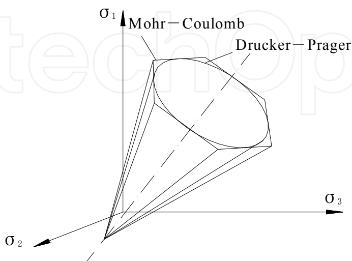
Fig. 1. Mohr–Coulomb & Drucker–Prager yield surface
