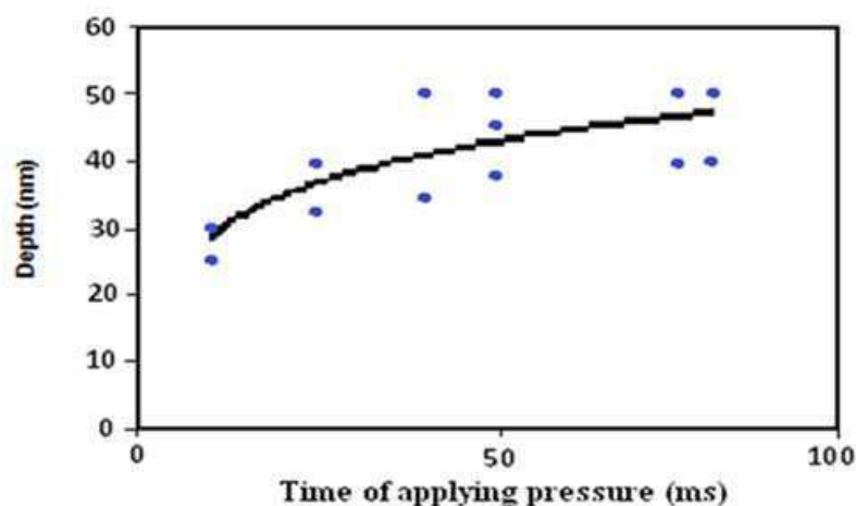
Fig. 12. Indentation depth dependence to time of applying pressure for PE substrate (Sadegh Hassani et al., 2008b), while applied normal force, scanning velocity and number of scratching cycle are 4\mu\text{N} , 140\text{ nm/s} , 10, respectively.
