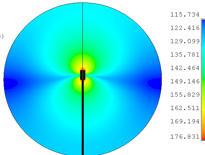
Fig. 11. Acoustic pressure pattern generated by the tip in the liquid
