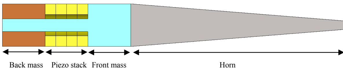
Fig. 1. General structure of a horn-type piezoelectric transducer
