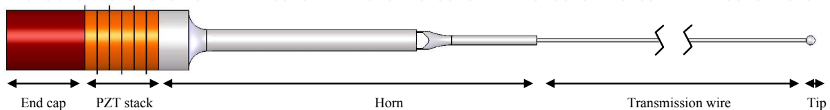
Fig. 9. Schematic illustration of the piezoelectric thrombolysis device
