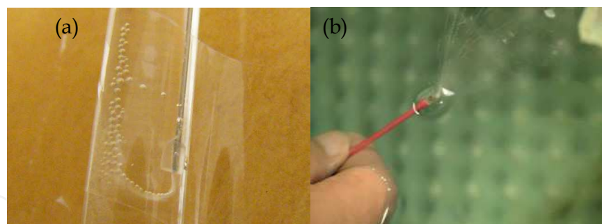
Fig. 12. Acoustic cavitation (a) and acoustic streaming (b)
