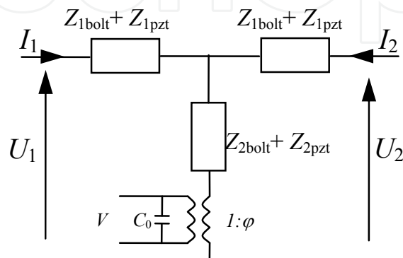
Fig. 3. Piezoelectric stack element (Lin, 2004b)
