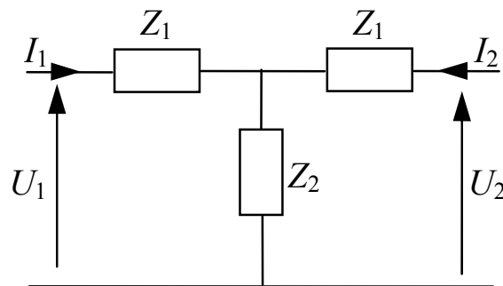
Fig. 2. Front and back mass elements
