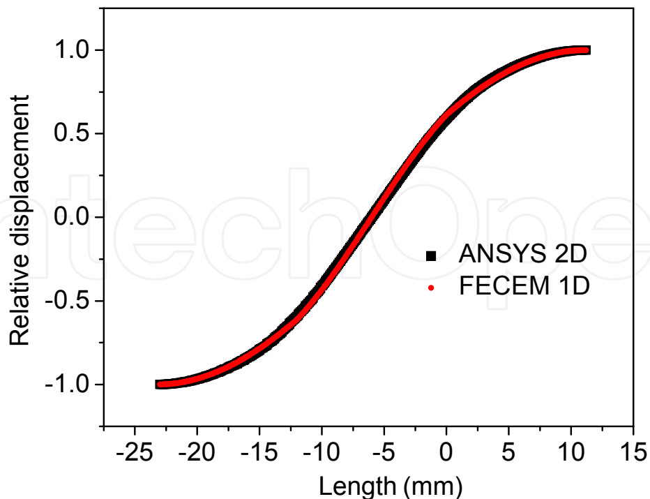
Fig. 5. Comparison of mode shape of Langevin transducer
