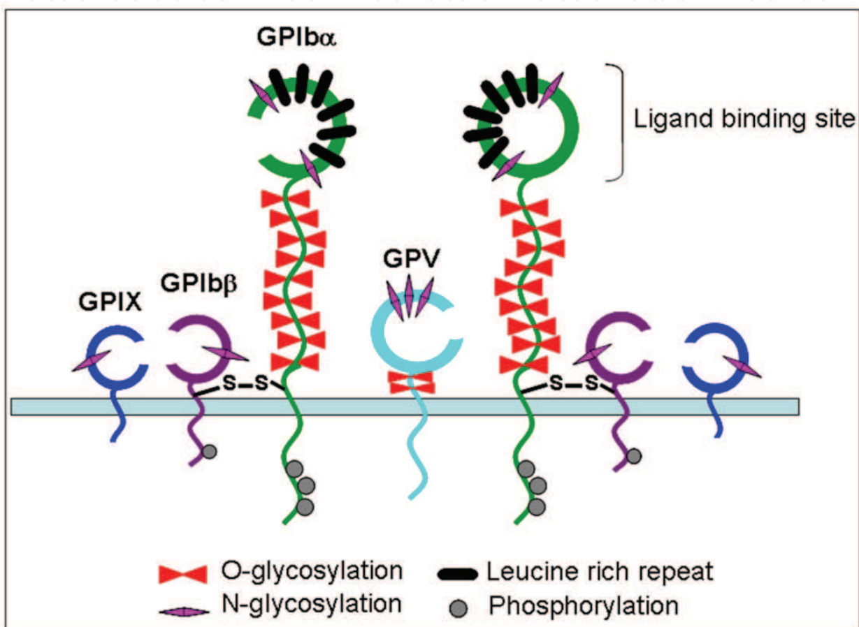
Fig. 1. GPIb-IX-V complex
