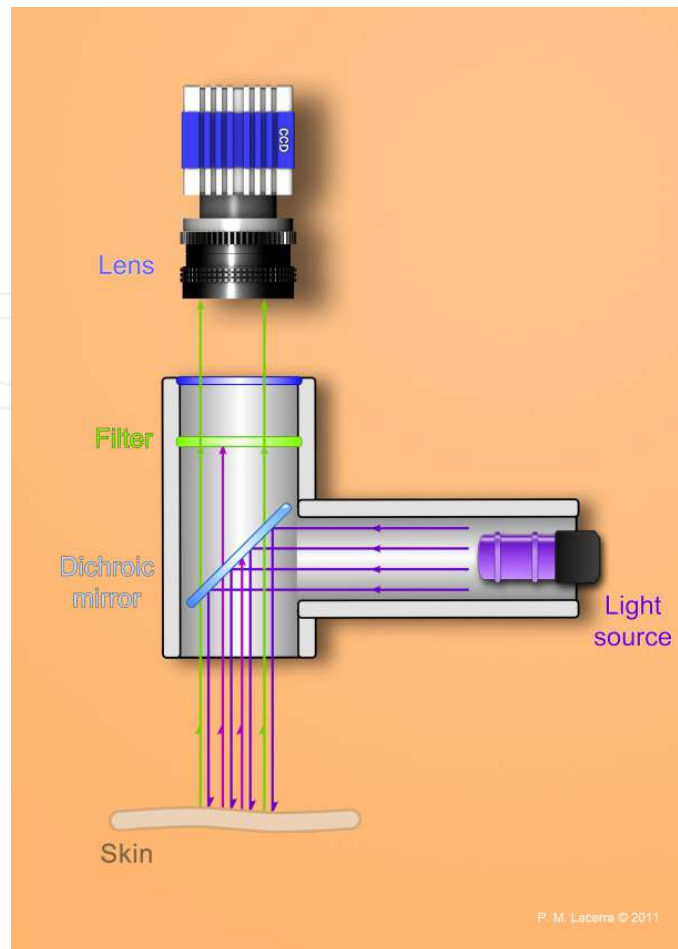
Fig. 4. Configuration of the fluorescence imaging device used.
