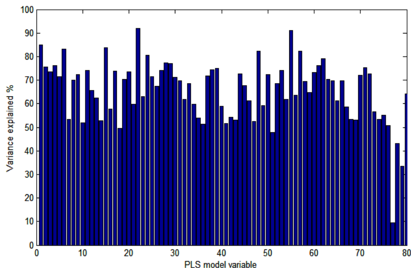
Fig. 8. Variance explanation for CCGT efficiency in multi-shaft unit
