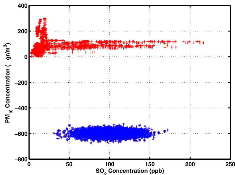
Fig. 2. Air pollution and synthetic cloud patterns.
